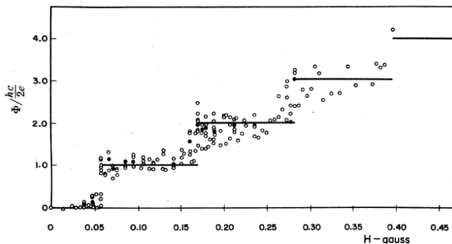
FIG. 2: Experimentally measured trapped flux threaded in a superconducting cylinder as a function of magnetic field, in which the cylinder was cooled below the superconducting transition temperature [9].
